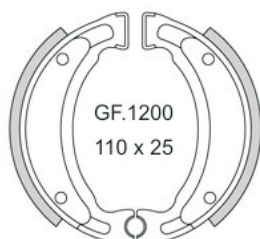
98.1134 Sinter Fr. 23.80
